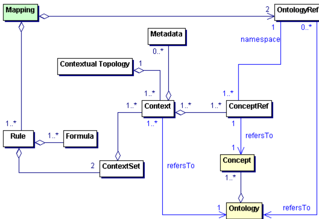
Semantic Translation meta-model
